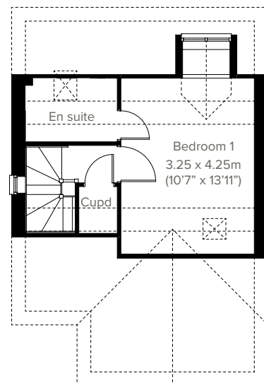
2ND FLOOR
