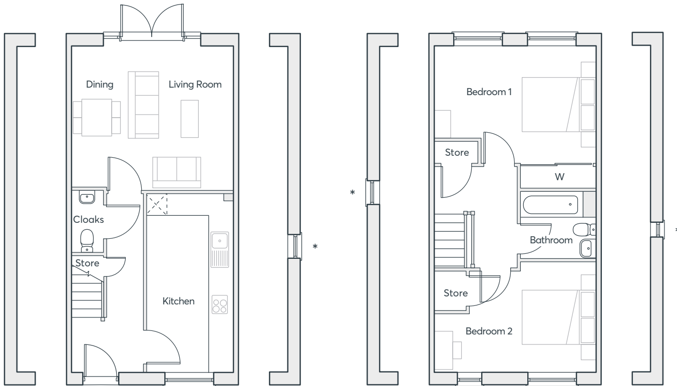
GROUND FLOOR
