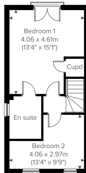
2ND FLOOR
