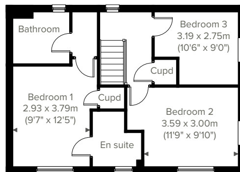
1ST FLOOR
