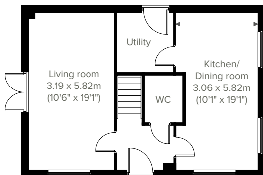
GROUND FLOOR
