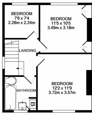
1ST FLOOR APPROX. FLOOR AREA 411 SQ.FT. (38.2 SQ.M.)
