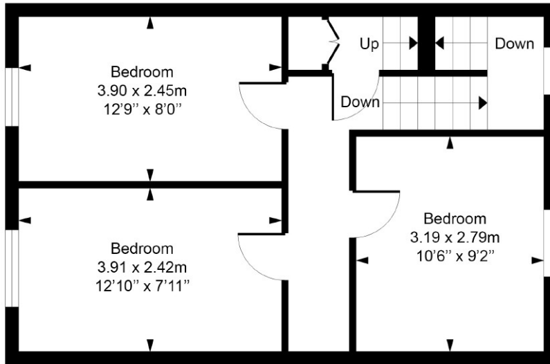
Second Floor
