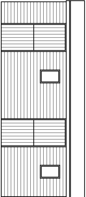
FRONT ELEVATION
