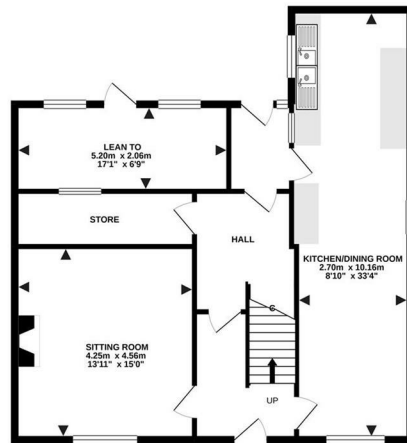
GROUND FLOOR 79.8 sq.m. (858 sq.ft.) approx.
