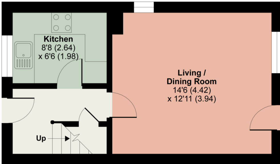
GROUND FLOOR
