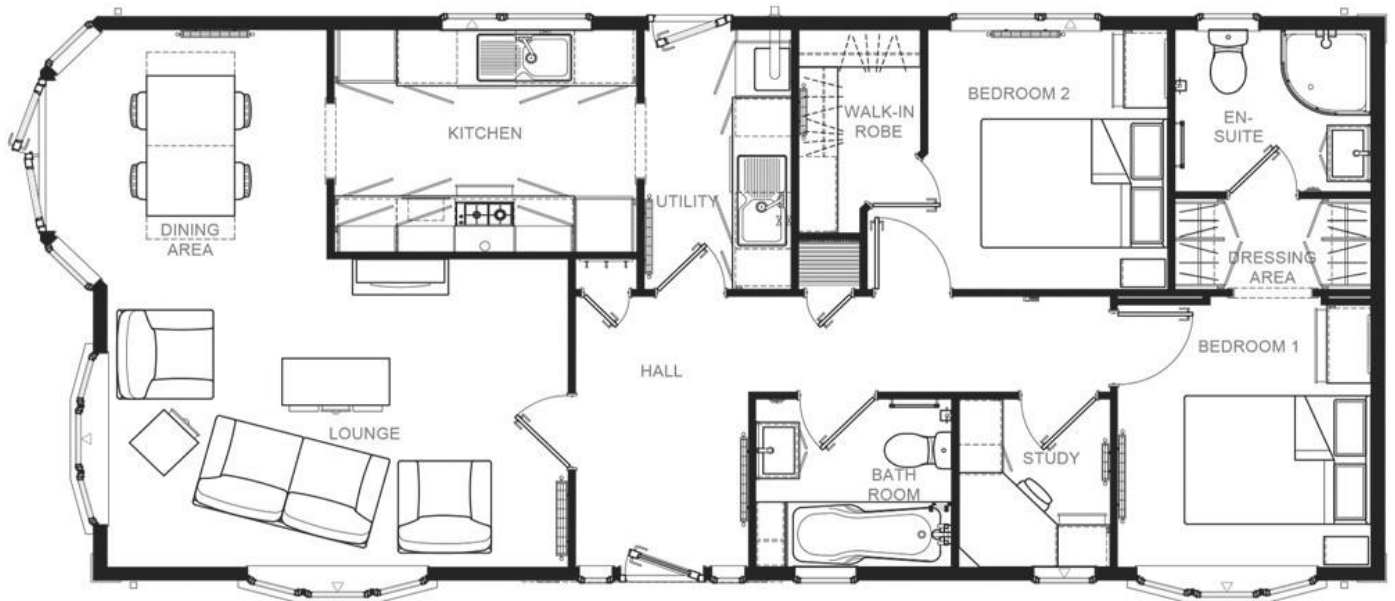
Sandringham 45x20 2DB Utility & Study
