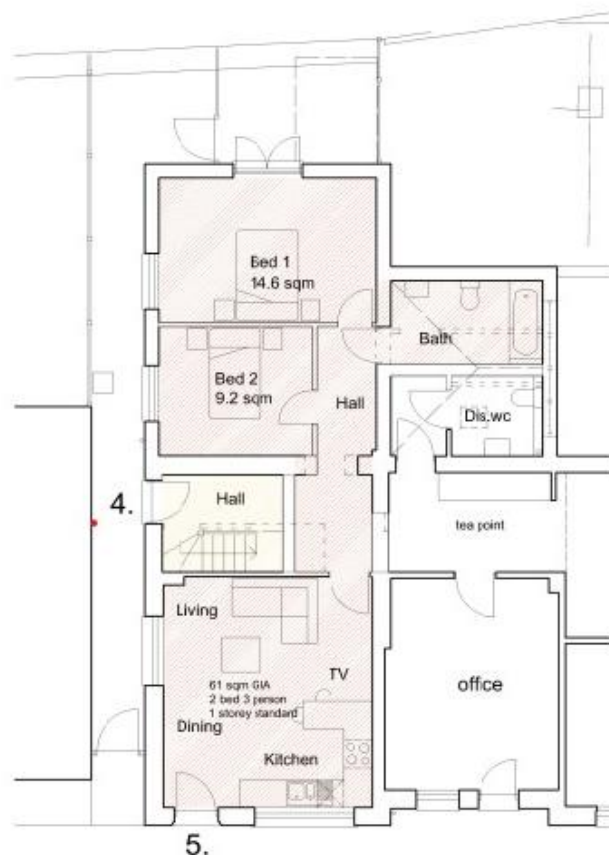
Proposed conversion - ground floor plan 1:100@A3
