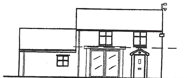
East Elevation
