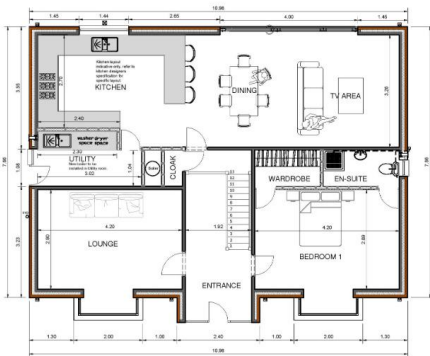
Ground Floor Layout (SCALE 1:50)
