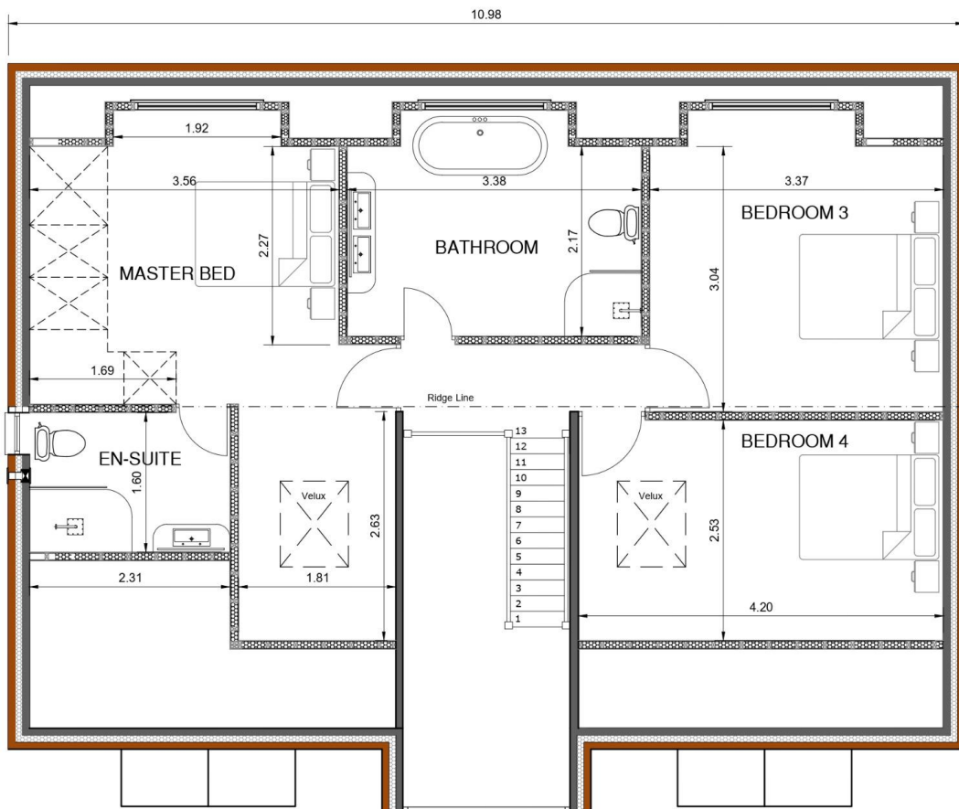
First Floor Layout (SCALE 1:50)
