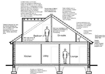
Section B-B (SCALE 1:50)
