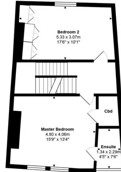
First Floor Area: 54.1 m 2 ... 582 ft 2
