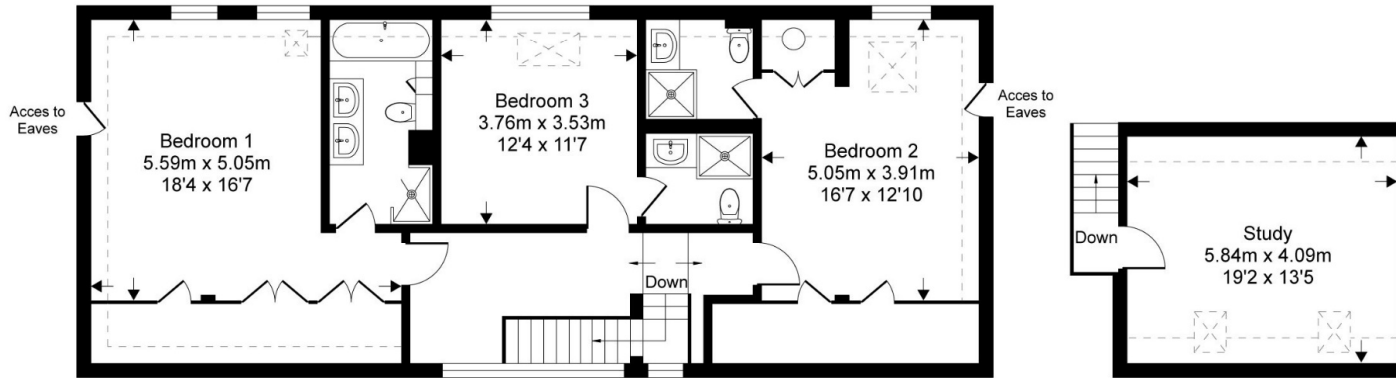
First Floor
