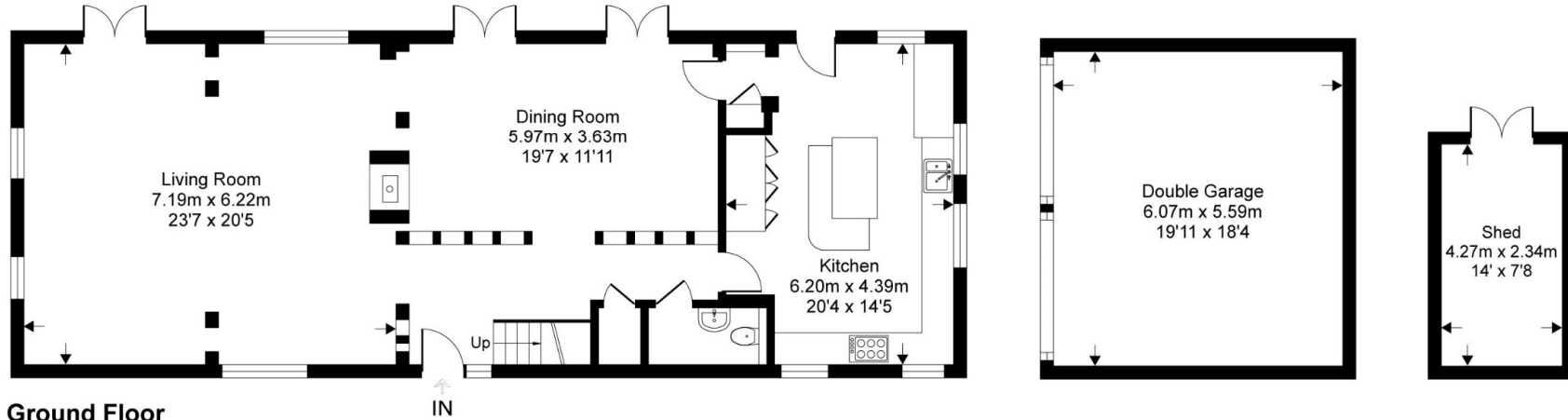
Ground Floor
