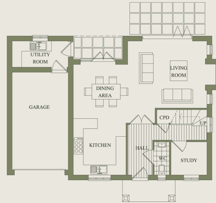
GROUND FLOOR PLAN THE CHESTNUT - PLOT 1
