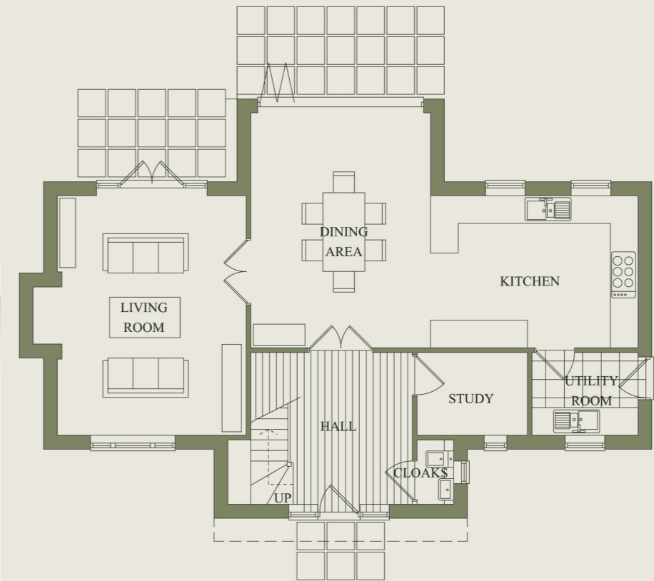
GROUND FLOOR PLAN THE CEDAR - PLOT 3
