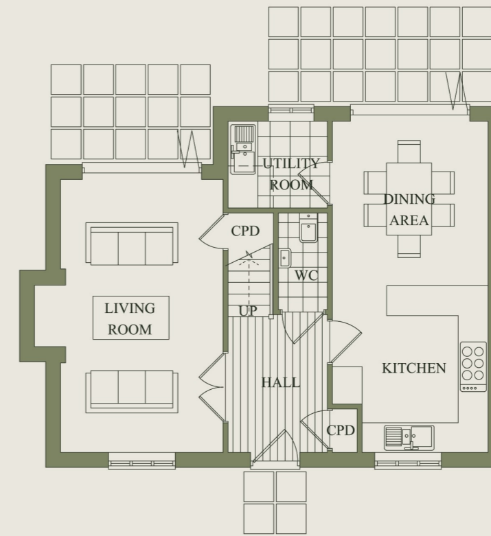
GROUND FLOOR PLAN THE ASPEN - PLOT 2
