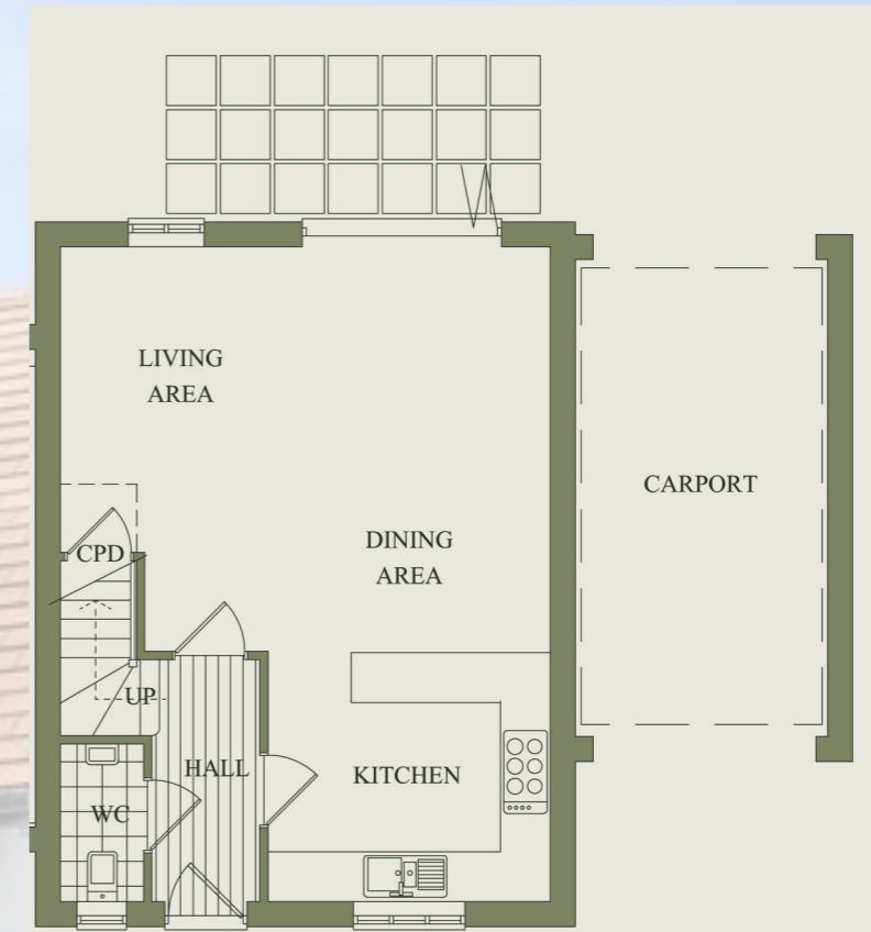
GROUND FLOOR PLAN THE MAPLE - PLOT 7
