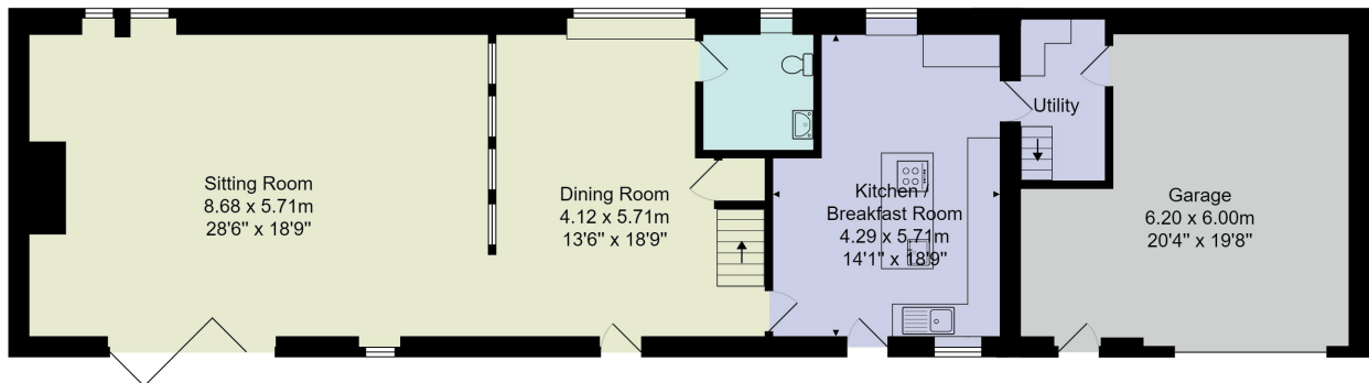
Ground Floor
