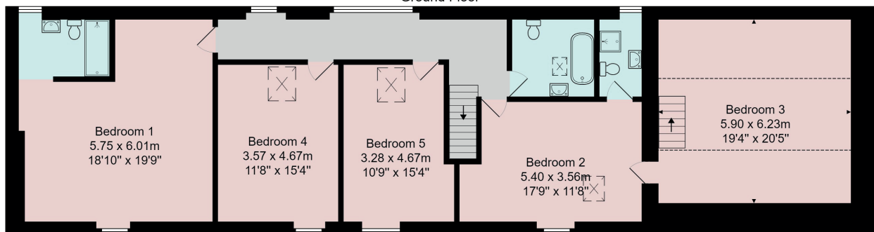
First Floor
