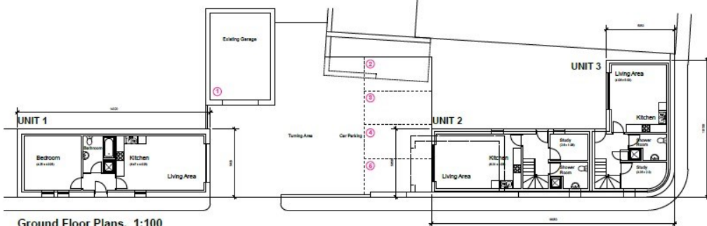
Ground Floor Plans. 1:100
