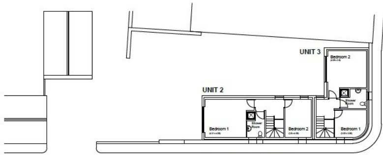
First Floor Plans. 1:100
