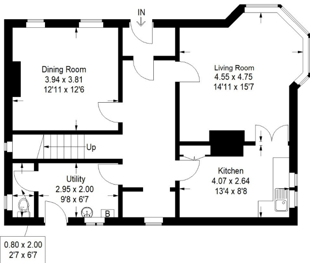
Ground Floor 73.6 sq m / 792 sq ft
