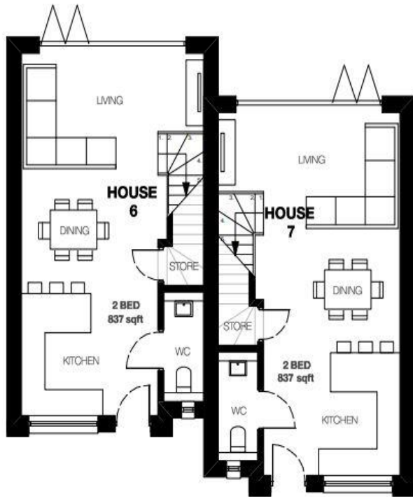
Houses 6-7 Ground floor plan
