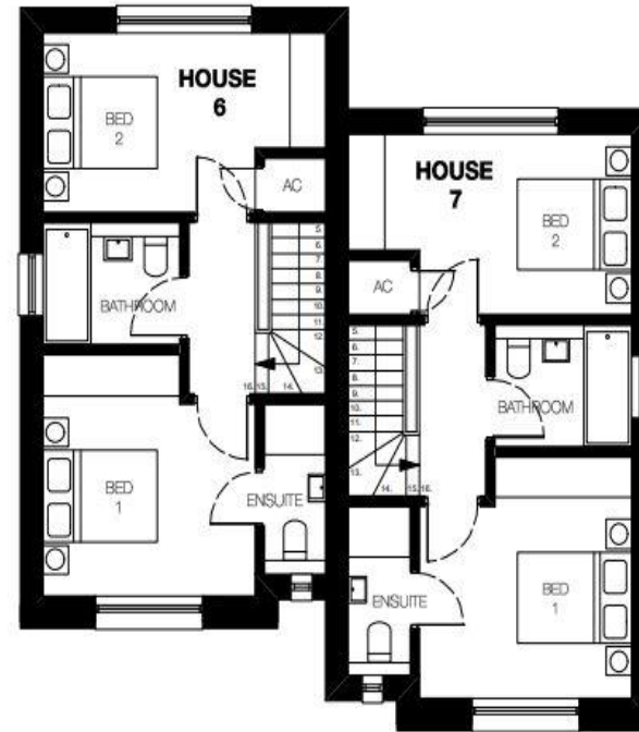
Houses 6-7 First floor plan
