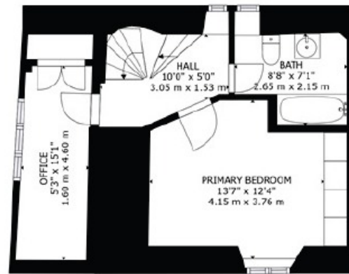
FLOOR 2
