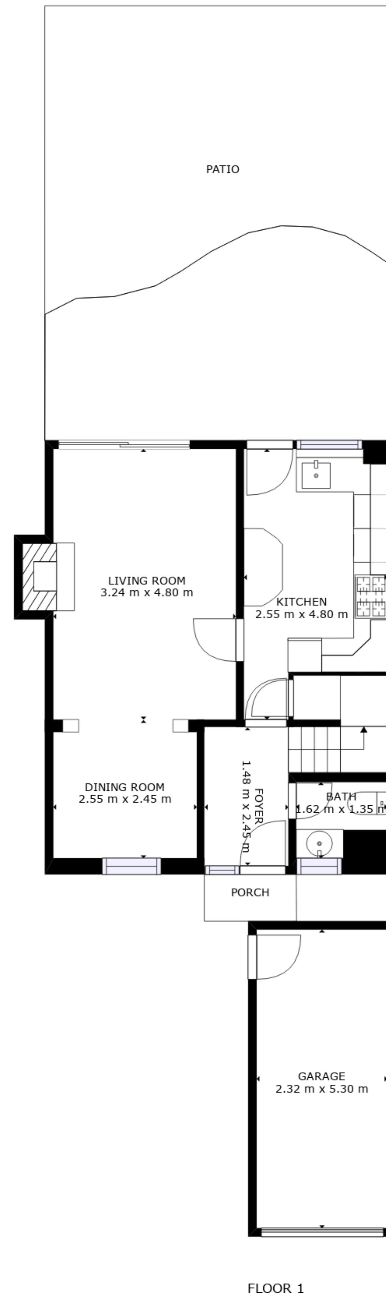
FLOOR 1
