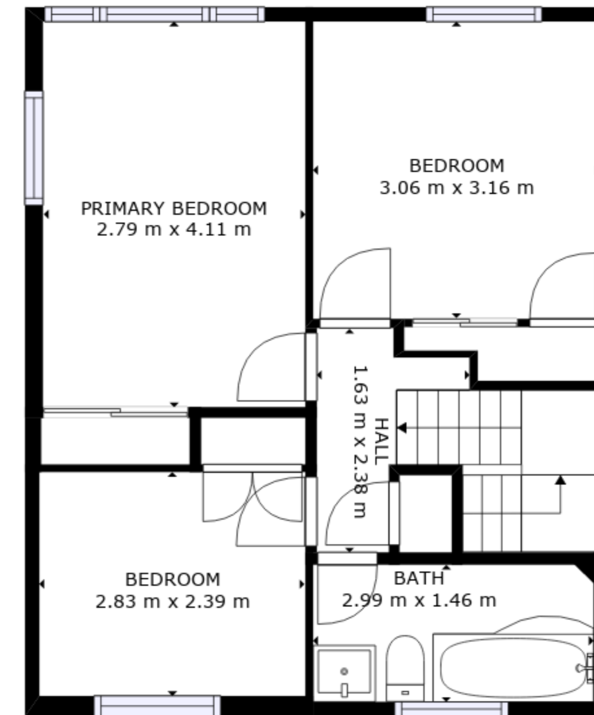
FLOOR 2
