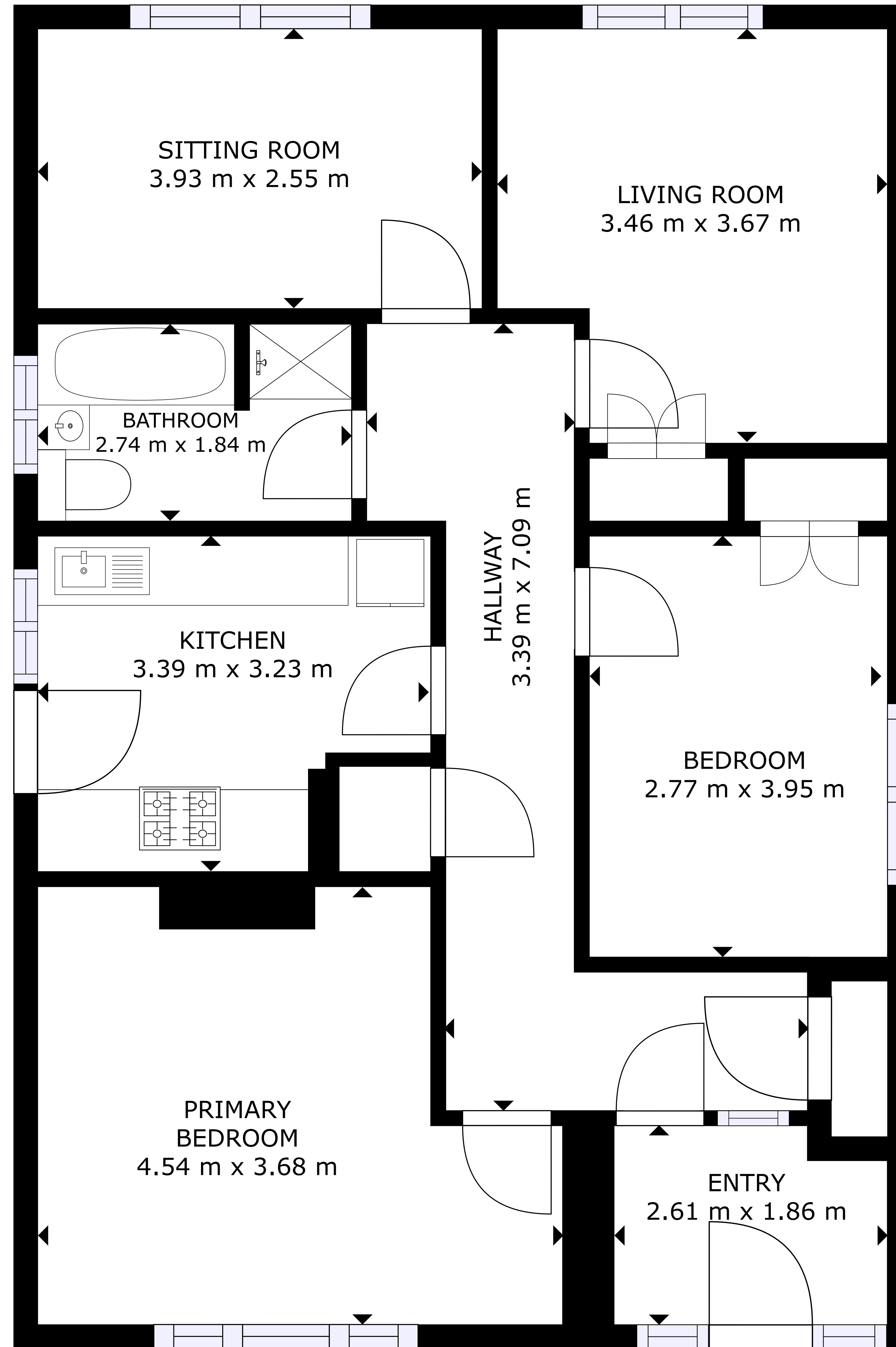
FLOOR PLAN
