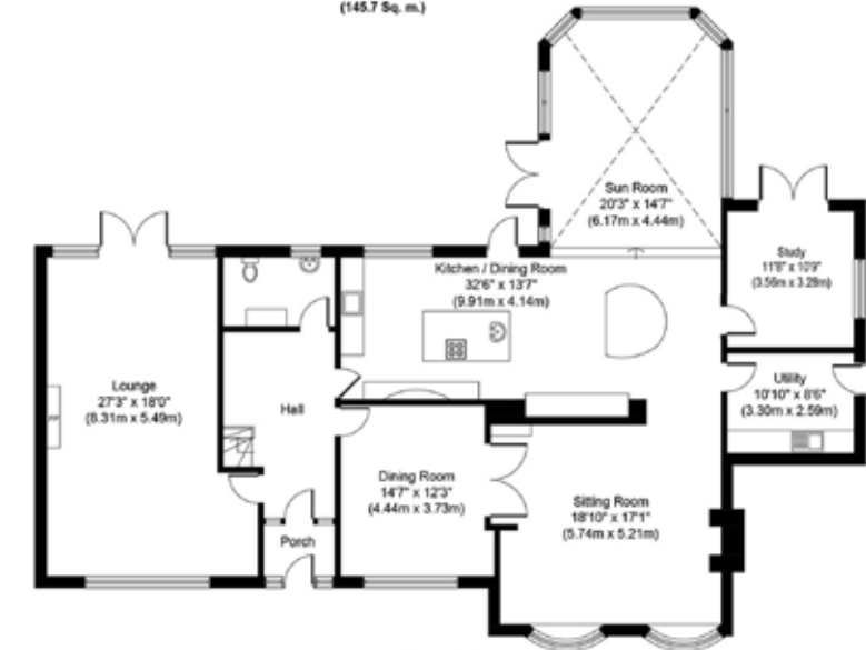
Ground Floor Approximate Floor Area 2182 Sq. ft. (202.7 Sq. m.)
