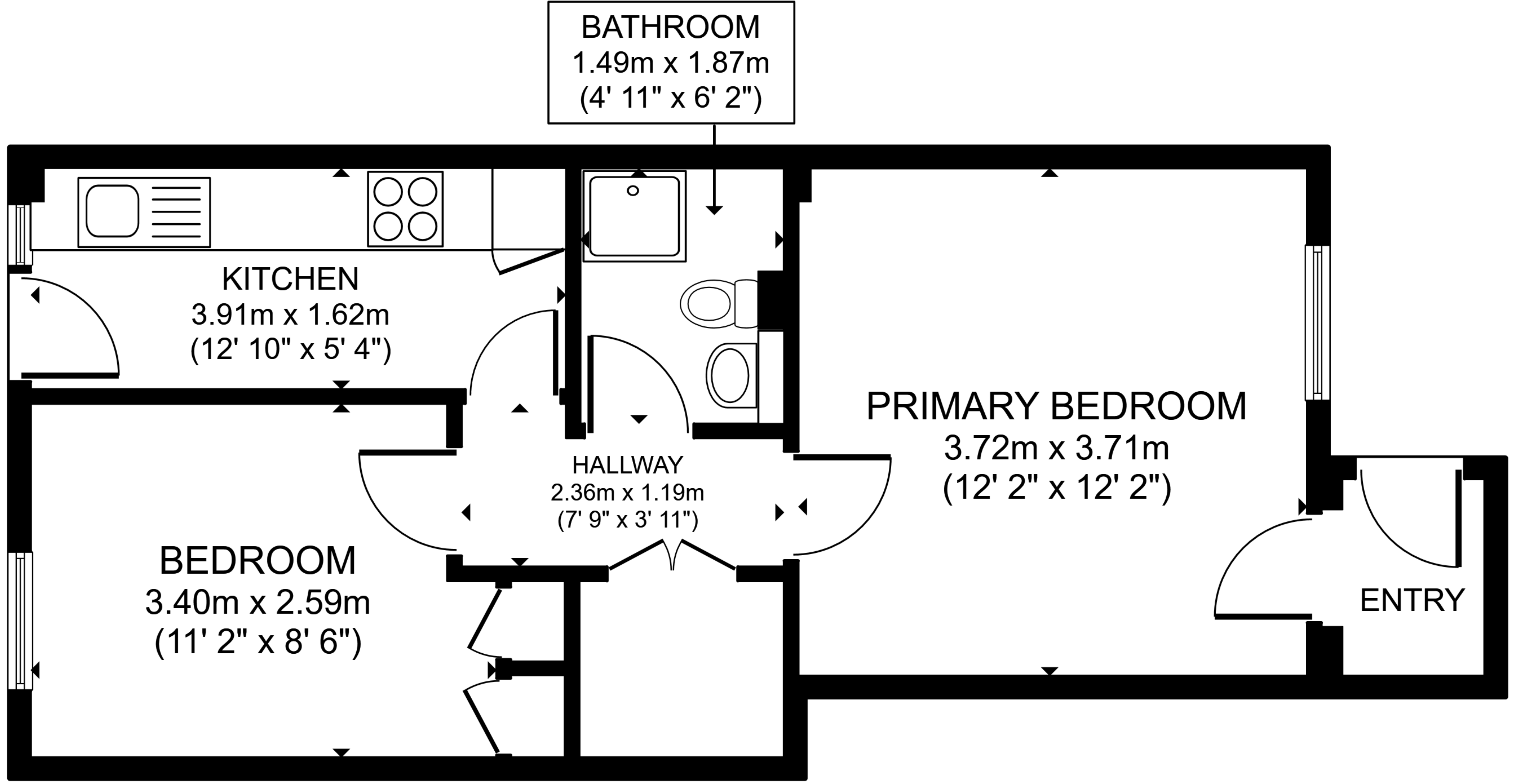
FLOOR PLAN
