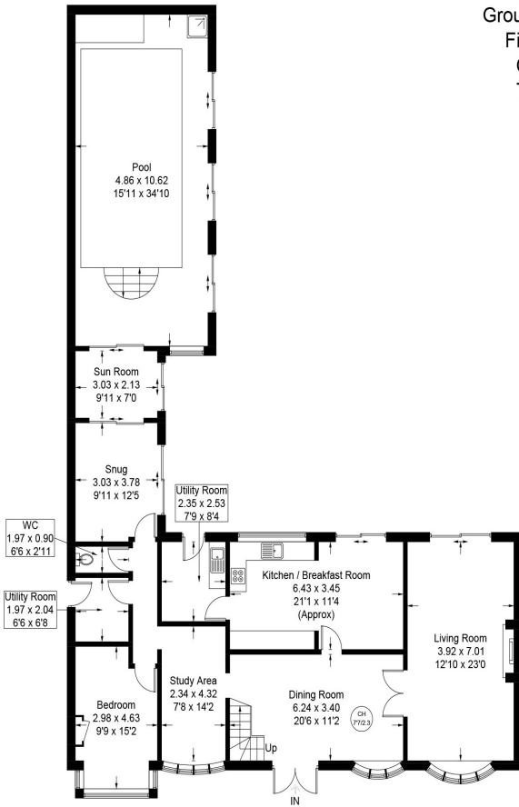
Ground Floor 187.4 sq m / 2017 sq ft
