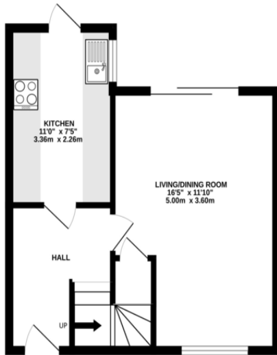
GROUND FLOOR 346 sq.ft. (32.2 sq.m.) approx.
