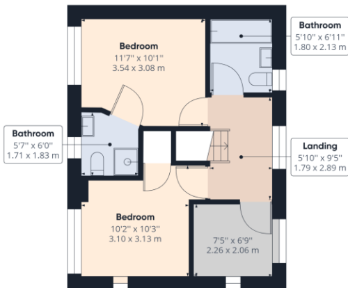
Floor 1 Building 1
