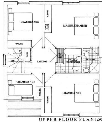
PROPOSED FLOORPLANS & ELEVATIONS U N I T No:1
