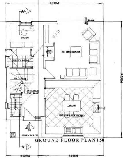
PROPOSED FLOORPLANS & ELEVATIONS U N I T No:1
