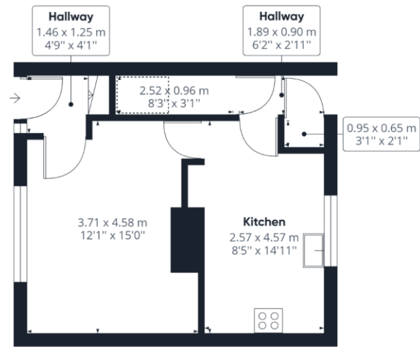
Floor 0
