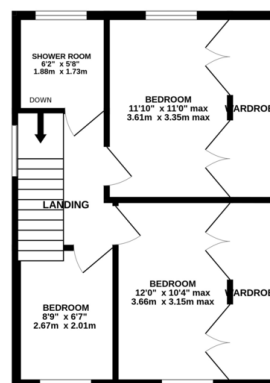
1ST FLOOR 396 sq.ft. (36.8 sq.m.) approx.
