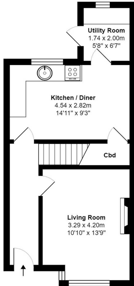
Ground Floor Area: 39.5 m 2 ... 426 ft 2
