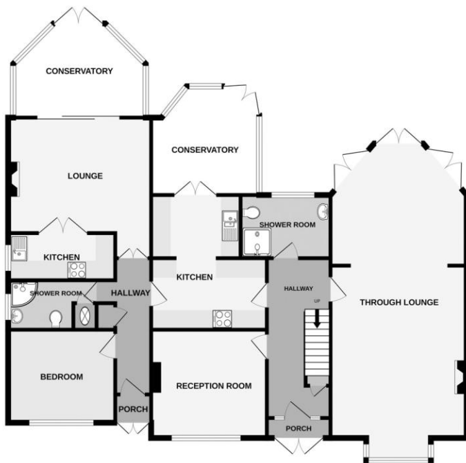
GROUND FLOOR 1533 sq.ft. (142.4 sq.m.) approx.
