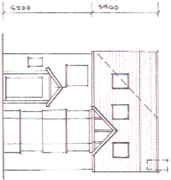
FRONT ELEVATION - WEST
