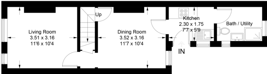
Ground Floor
