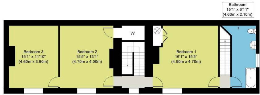
First Floor Approximate Floor Area 934 sq. ft (86.79 sq. m)
