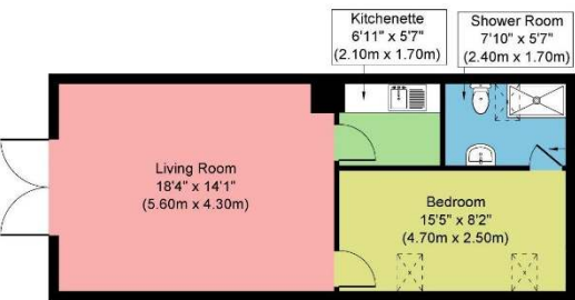
Annexe Approximate Floor Area 486 sq. ft (45.22 sq. m)
