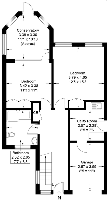
Ground Floor (Including Garage) 78.1 sq m / 841 sq ft
