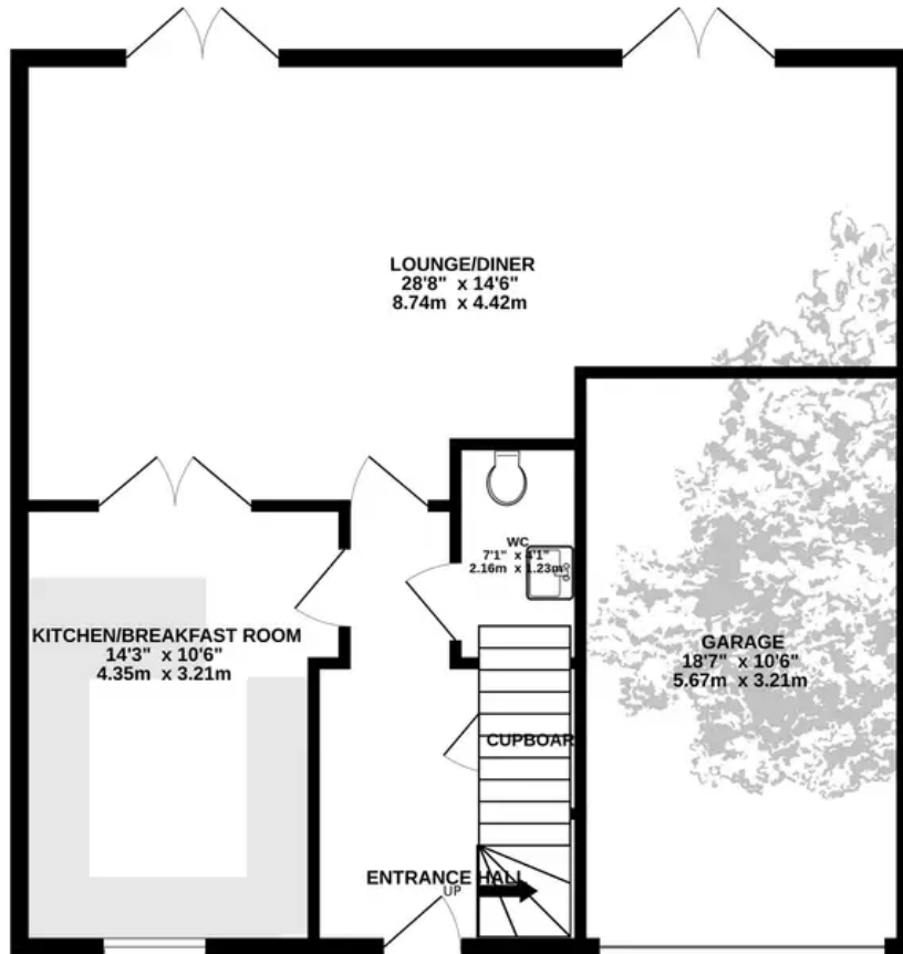
GROUND FLOOR UNIT 1 916 sq.ft. (85.1 sq.m.) approx.
