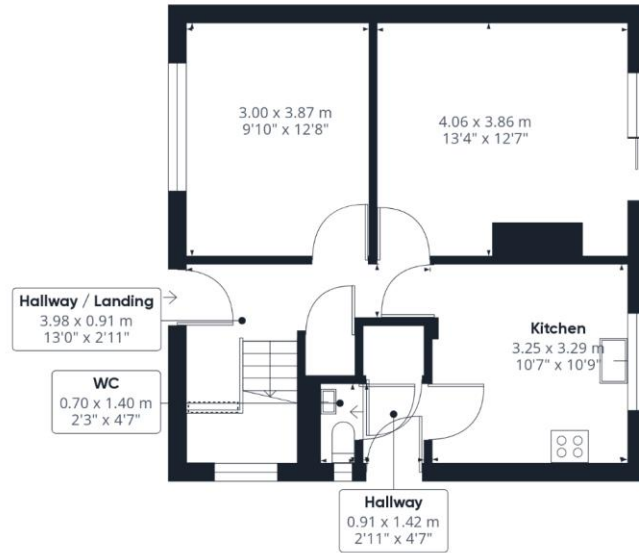
Floor 0
