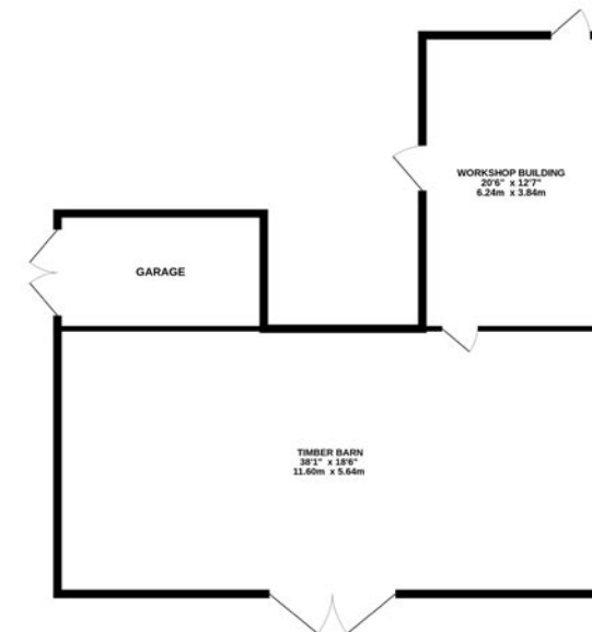
TOTAL FLOOR AREA: 1078 sq.ft. (100.1 sq.m.) approx.
