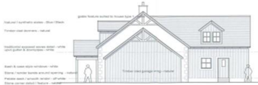
Side (North) Elevation 1:100
