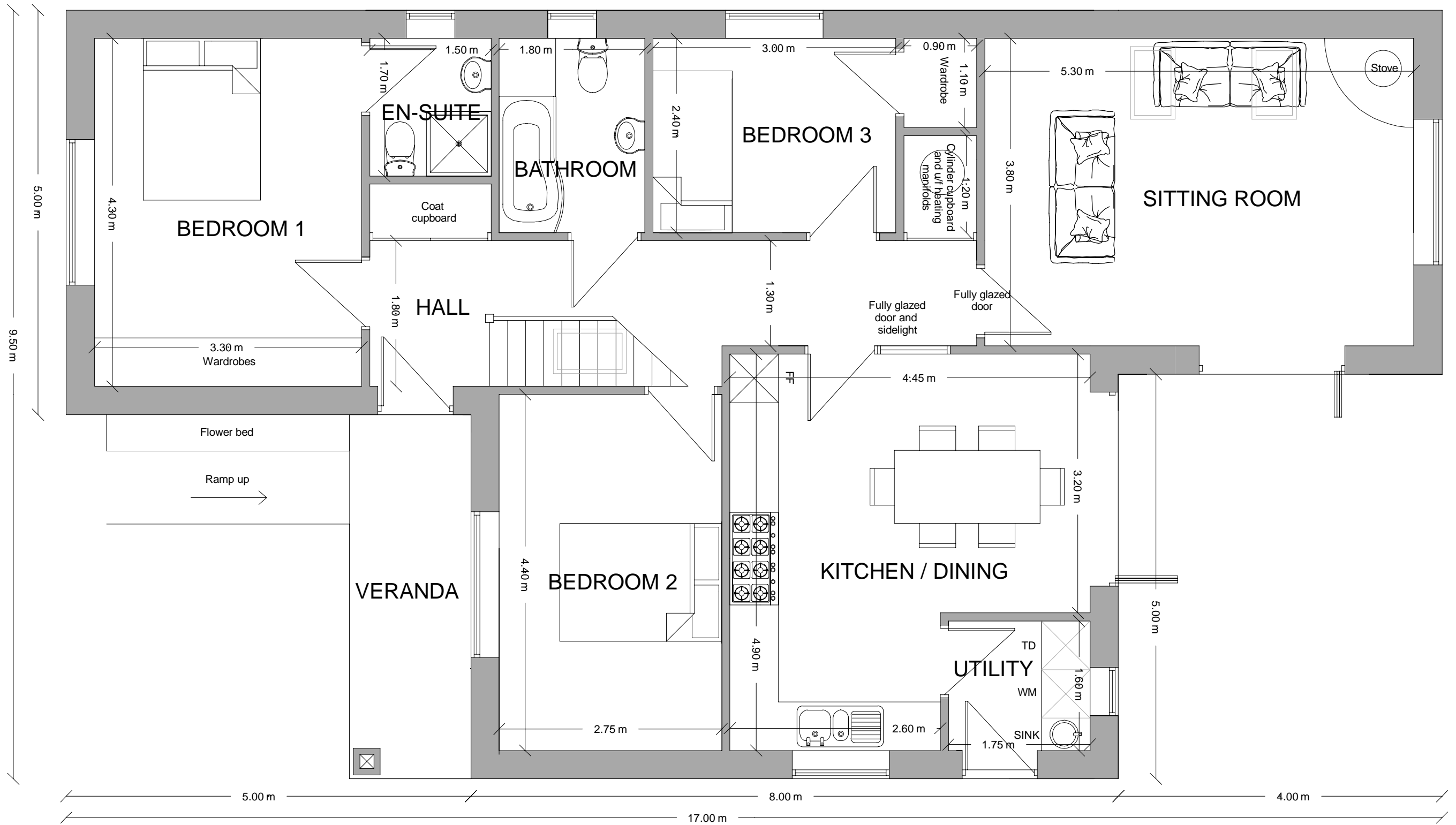
PROPOSED GF LAYOUT 1:50
