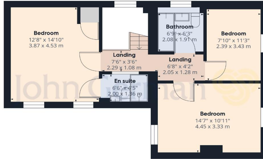
Floor 1 Building 1
