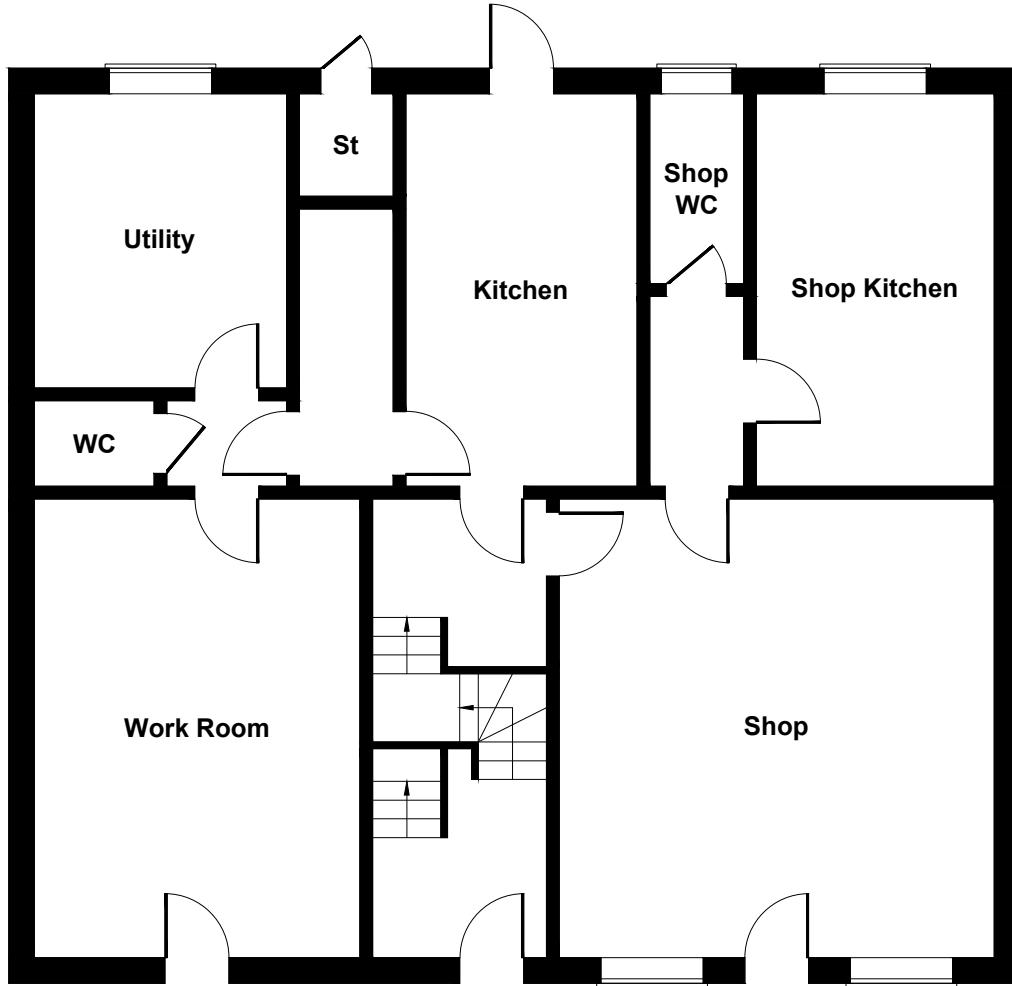
GROUND FLOOR
