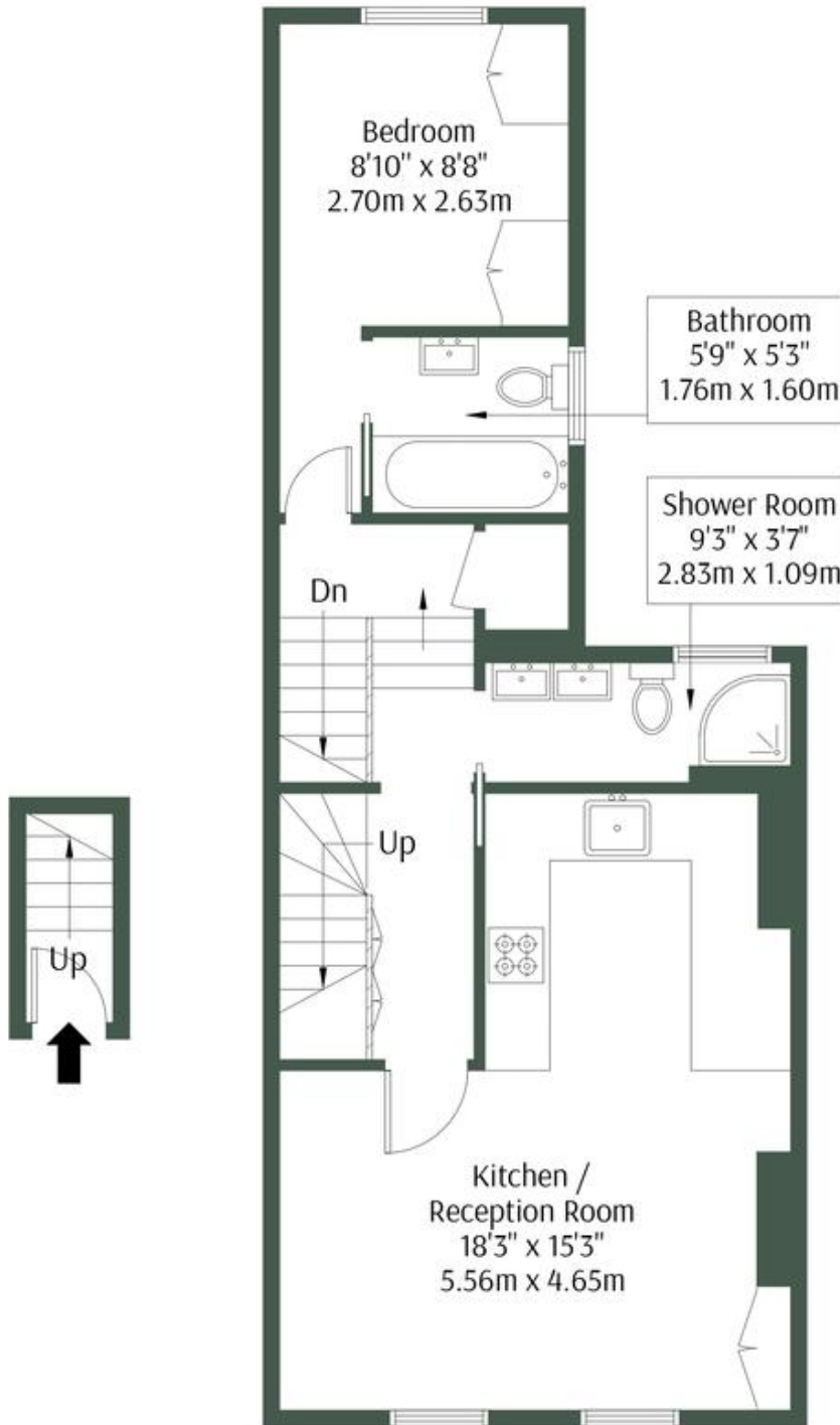
Ground Floor
