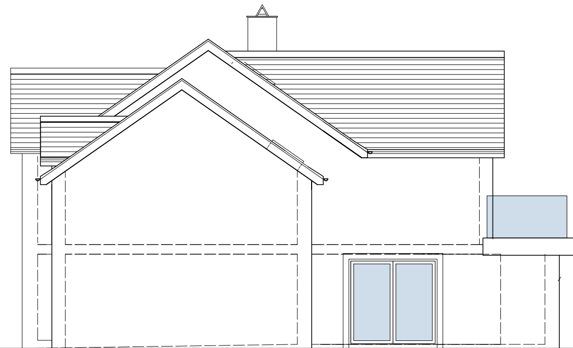
East South Easterly Facing Side Elevation
