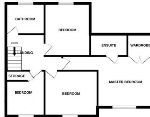
1ST FLOOR
