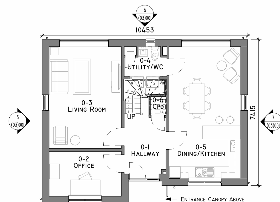
1 GROUND FLOOR PI 1 : 100
