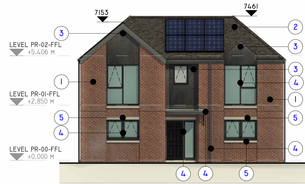
4 ELEVATION P1 - FRONT 1 : 100
