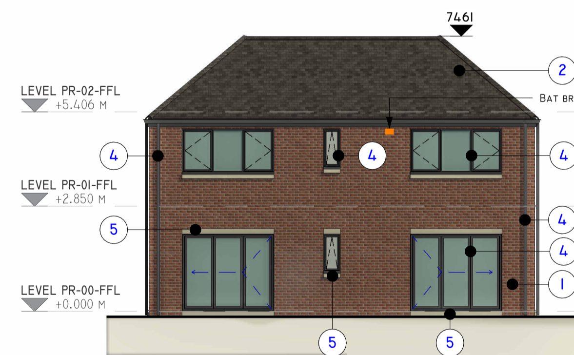
6 ELEVATION P3 - REAR 1 : 100
