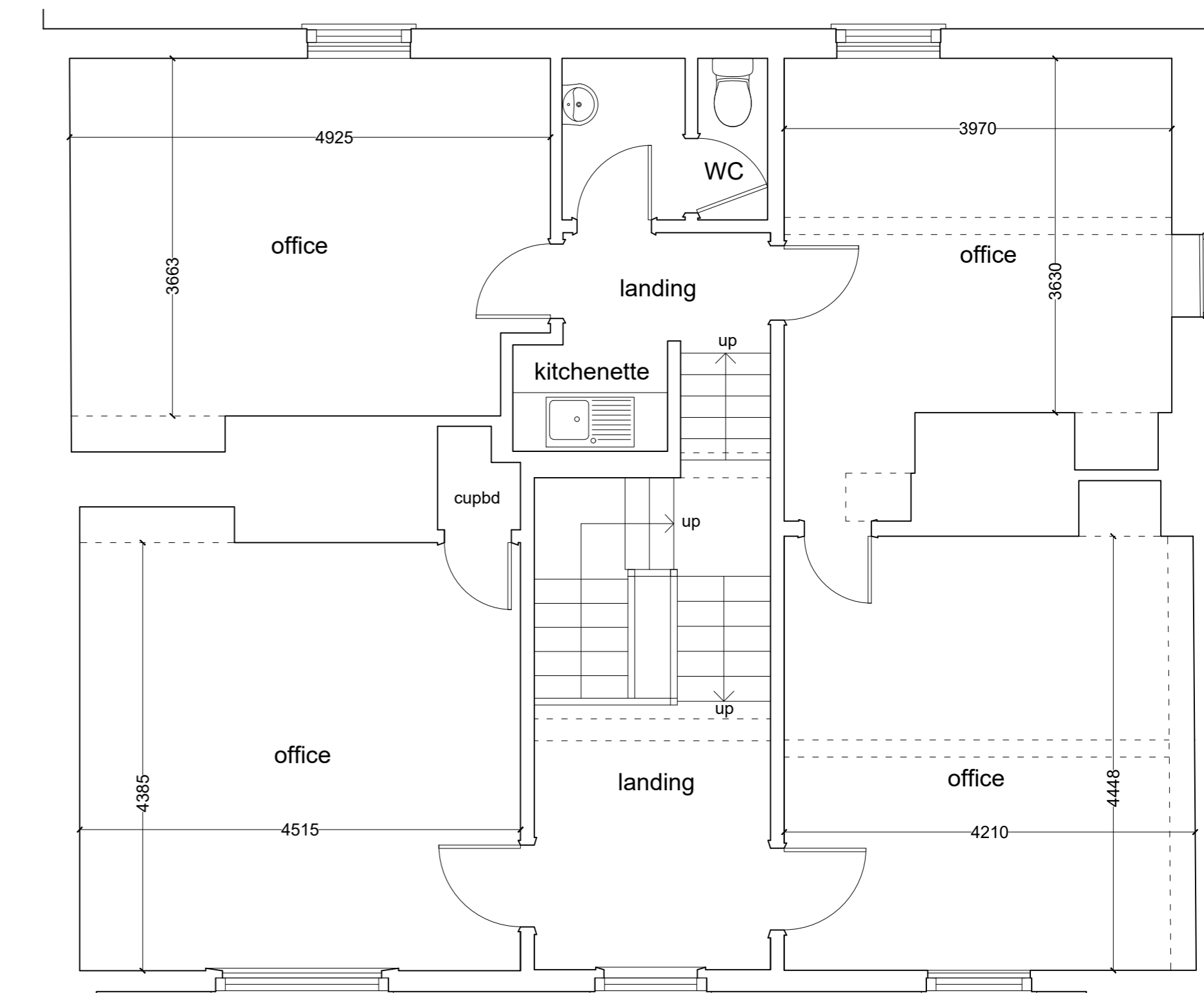
7 Market Place, Brigg First Floor Plan
