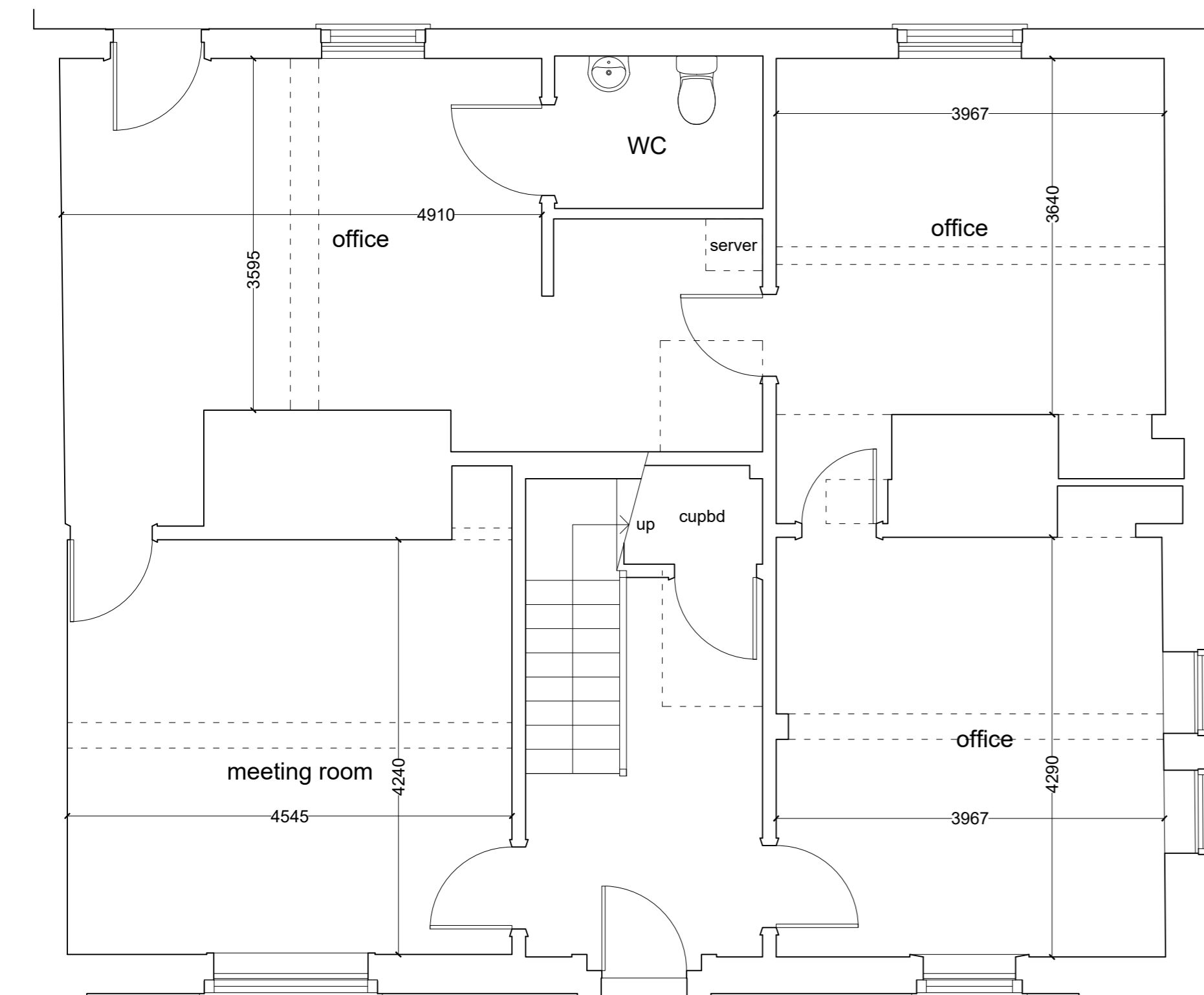
7 Market Place, Brigg Ground Floor Plan
