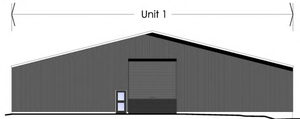
EAST ELEVATION
