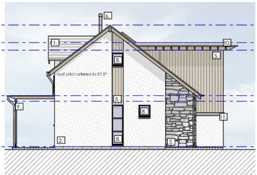
Proposed East Elevation Plan - scale 1:100
